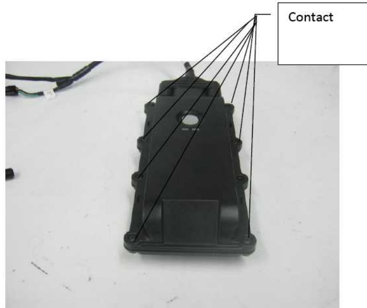
Figure 8. ESD Test Points
