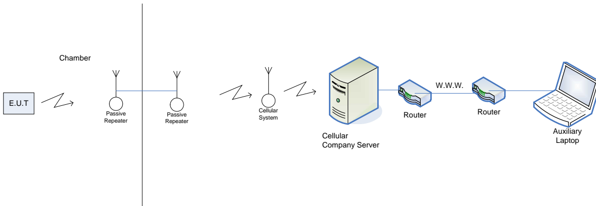
Figure 1. Test Set-up
