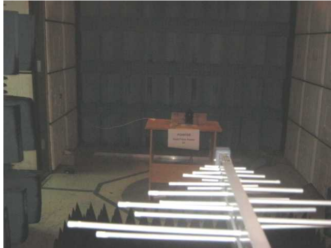
Figure 13. Immunity to Radiated Field Test
